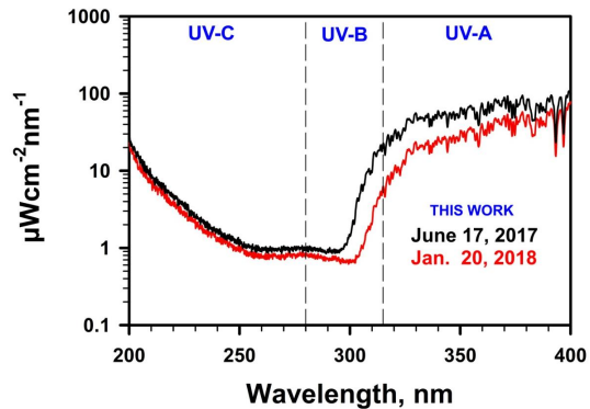
Fig. 3. Examples of our solar spectral irradiance measurements
