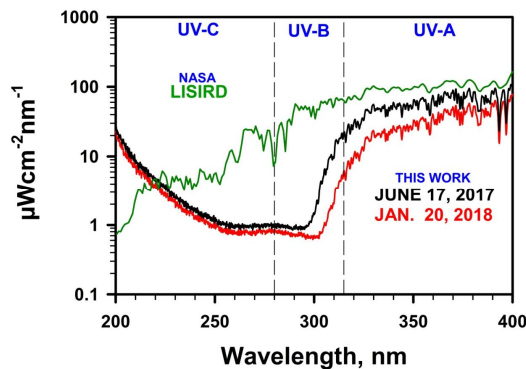
Fig. 6. Comparison of our UV solar spectral irradiance with NASA's LISIRD satellite-derived solar spectral irradiance at the top of the atmosphere [31]
