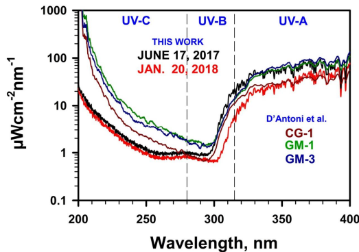
Fig. 5. Comparison of our solar spectrometric measurements with those of D’Antoni et al. [25]. Note the commonality of shape of the curves in the UV-C region of the spectrum
