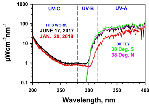
Fig. 4. Comparison of our solar spectral irradiance measurements with those of Diffey [22]
