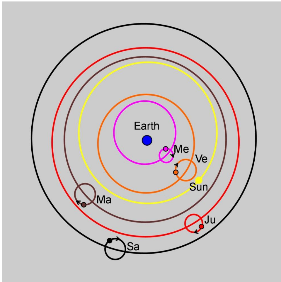
Figure 1. Epicycles were able to explain apparent retrograde motion of planets in the problematic Earth-centered Ptolemaic universe paradigm.
