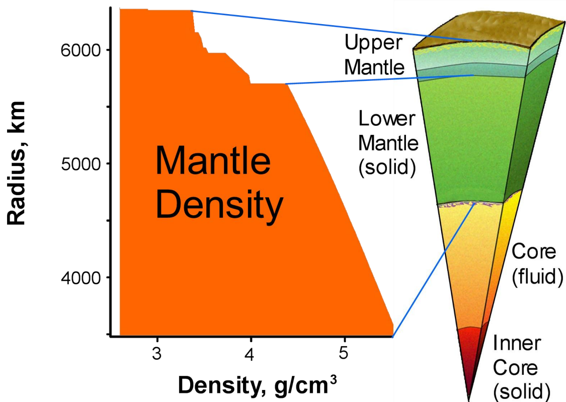
Figure 3. Density as a function of radius in the Earth's mantle [15].
